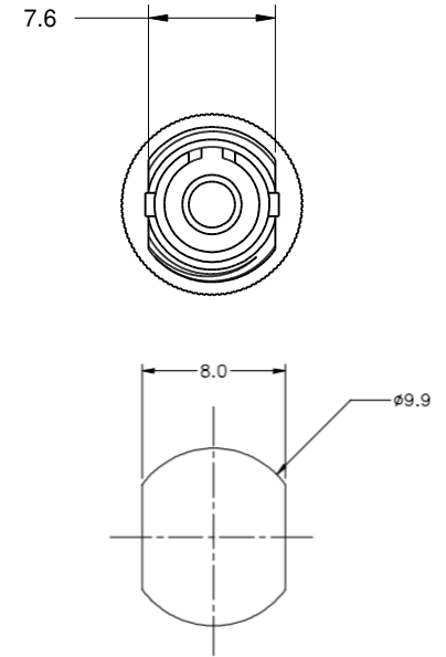
SUGGESTED MOUNTING PANEL CUTOUT
